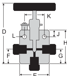
Three Way Valves One Pressure Connection
